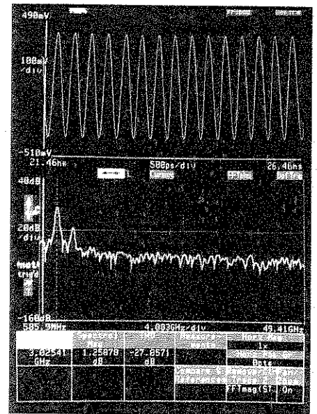
Figure 2. FFT display and measurements in the 11801B offer additional analysis power to the engineer or scientist.
