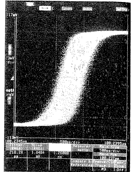
Figure 1. Direct and automatic jitter, noise and rise time measurement using the statistical measurement mode.
