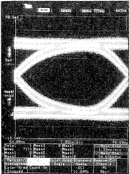
Figure 3. Predefined Telecom masks make verifying digital stream conformance simple.
